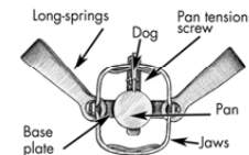
Figure 1a. Longspring Trap
